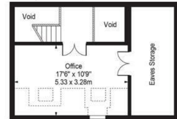
Fourth Floor
